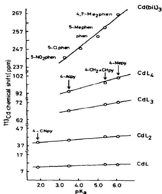
Fig. 11. Plot of ^{113}\text{Cd} chemical shifts of Cd complexes with 4-substituted pyridines (L) and 1,10-phenanthroline and its derivatives (biL) versus the pK a values of the ligands (ref. 39).
