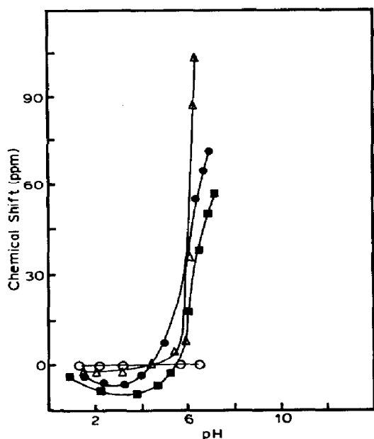
Fig. 15. ^{113}\text{Cd} chemical shift as a function of pH for 0.3 M \text{Cd}(\text{ClO}_4)_2 and 0.6 M methylamine ( \blacklozenge ), glycine ( \bullet ), glycine methyl ester ( \blacktriangle ), and N,N -dimethylglycine ( \blacksquare ). From ref. 100.
