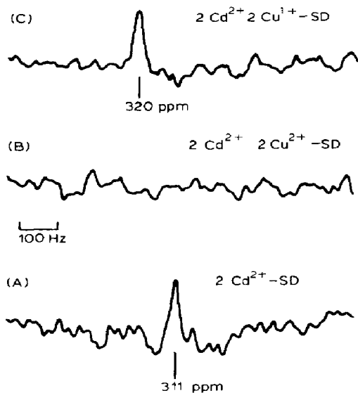
Fig. 24. ^{113}\text{Cd} NMR spectra of Cd-substituted superoxide dismutase. (A) \text{Cd}_2(\text{SD}) , with Cd in the equivalent Zn sites; (B) \text{Cd}_2\text{Cu}(\text{II})_2(\text{SD}) , (no signals are observed due to line broadening effects of paramagnetic \text{Cu}(\text{II}) ); (C) \text{Cd}_2\text{Cu}(\text{I})_2(\text{SD}) . From ref. 18.
