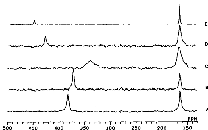
Fig. 8. ^{113}\text{Cd} NMR spectra obtained for \text{DMSO}-d_6 solutions (ambient temperature) containing \text{Cd}(\text{NO}_3)_2 (0.1 M), (\text{BzCH}_2)_3\text{N} (L1, 0.1 M), and X anions (0.05 M; \text{X} = \text{Cl}^- (A), \text{Br}^- (B), \text{I}^- (C), l-cysteine (D), \text{PhS}^- (E)). The upfield signals at \delta 163 and the downfield signals are for \text{Cd}(\text{L1}) and \text{Cd}(\text{L1})\text{X} , respectively (ref. 59).
