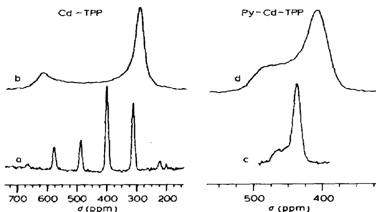
Fig. 1. Solid-state CP ^{113}\text{Cd} NMR spectra of \text{Cd}(\text{TPP}) (a and b) and its ^{15}\text{N} -pyridine adduct \text{pyCd}(\text{TPP}) (c and d). (a) and (c) MAS spectra; (b) and (d) powder patterns for the axially symmetric shielding tensors. From ref. 27.
