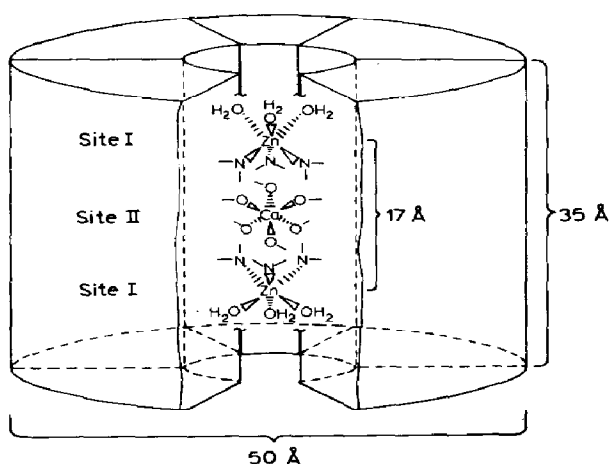
Fig. 19. Representation of the insulin hexamer showing the proposed Ca and Zn binding sites (ref. 118).
